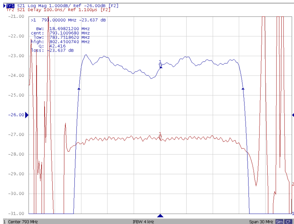
Fig2. Horizontal: 3MHz/Div Vertical: 1dB/Div
